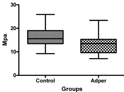
FIGURE 1. Box plots for shear bond strength (in MPa) of experimental groups.
